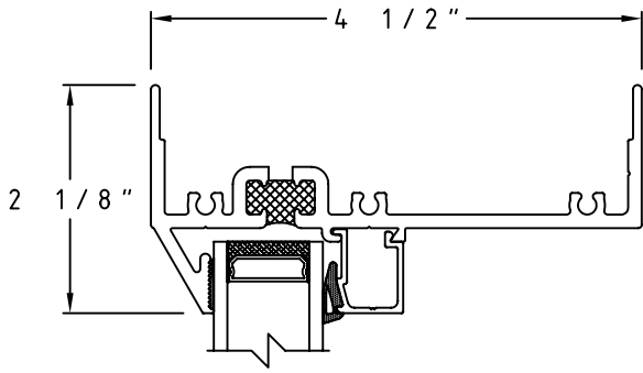
① Head Detail
