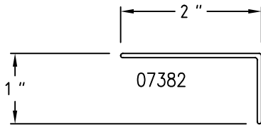
SC2 1" x 2" x 0.060" Stool Cover
